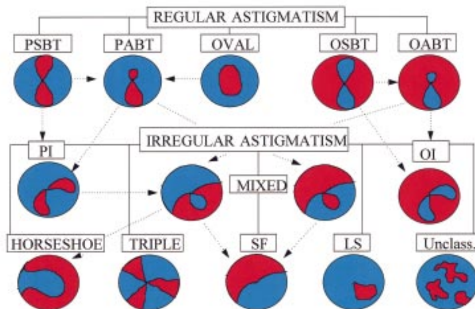
Figure 1 Proposed videokeratography pattern classification scheme. PSBT=prolate symmetric bow tie, PABT=prolate asymmetric bow tie, OSBT=oblate symmetric bow tie, OABT=oblate asymmetric bow tie, PI=prolate irregular, OI=oblate irregular, SF=steep/flat, LS=localised steep. Most of the patterns can be seen as a continuum, with some of them changing into different patterns (arrows) after manipulation of post-PKP astigmatism, by removal or adjustment of sutures. Blue and red colours imply flat and steep areas respectively, as in the conventional topographic map representation.
