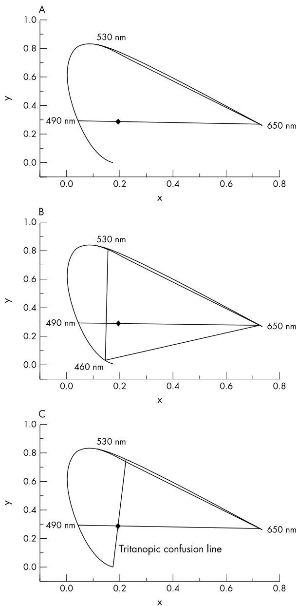
Figure 1 Chromaticity diagrams illustrating the principle of colour matching to establish the presence of S-cones. (A) The possible colours obtainable using mixtures of 530 nm and 650 nm light and a separate mixture of 490 nm and 650 nm light. The circle on the 490–650 nm line indicates the position of the test colour. For this combination of primaries, no colour match is possible for a trichromatic subject. (B) This shows that the addition of 460 nm light to 530 nm and 650 nm allows a trichromatic subject to achieve a colour match. (C) Shows that in tritanopia, a colour match is possible as the ratio of 530 nm to 650 nm light can be adjusted so that both colours lie on a tritanopic confusion line.
