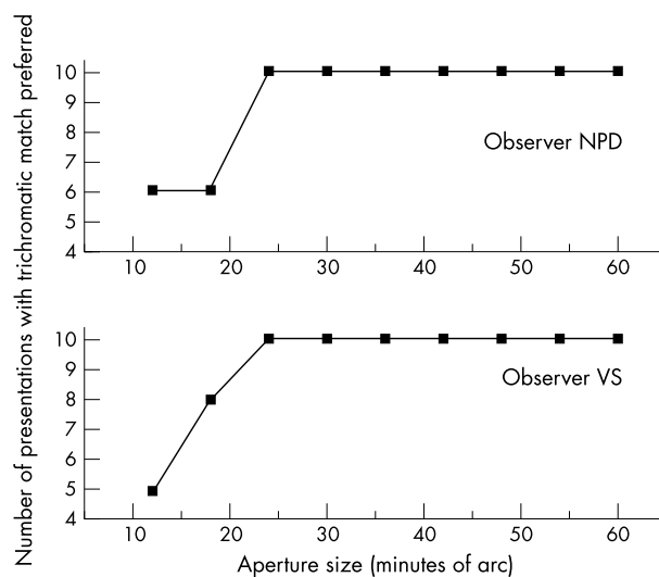
Figure 2 Results of forced choice presentations of dichromatic and trichromatic colour matches as a function of aperture size for observers NPD and VS. Note that with aperture sizes below 20' of arc the forced choice response approaches five, which would be expected by chance (that is, the observers have reached a tritanopic zone)
