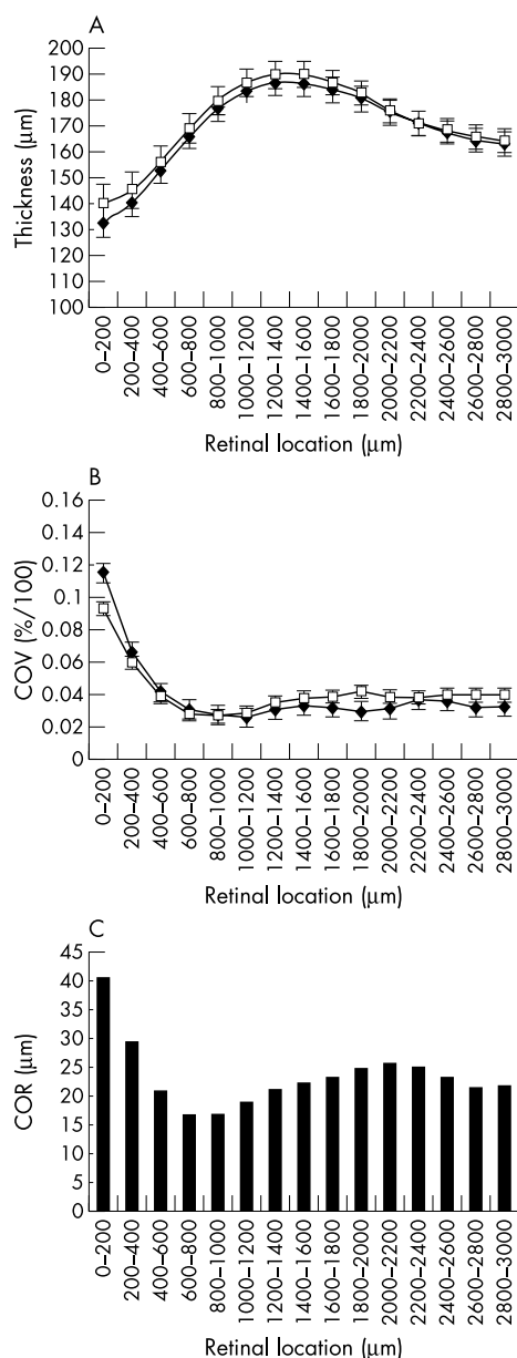
Figure 2 (A) Group mean profile of retinal thickness (0–3000 μm) derived using the circular band analysis for visits 1 (solid circle) and 2 (open square). (B) Group mean profile of COV derived using the circular band analysis for visits 1 (solid circle) and 2 (open square). (C) Bar chart showing group mean COR derived using the circular band analysis. For graphs A and B, the error bars represent plus or minus 1 standard error of the mean (COV = coefficient of variation. COR = coefficient of repeatability).
