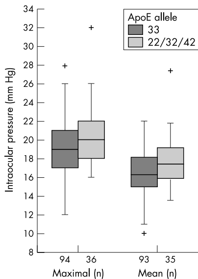
Figure 1 Maximal and mean IOP of the 24 hour diurnal curve of 130 individuals (normal controls, OHT, pre-OAG, and OAG); + cases with more than 1.5 box lengths from the upper or lower edge of the box. The box length is the interquartile range.
