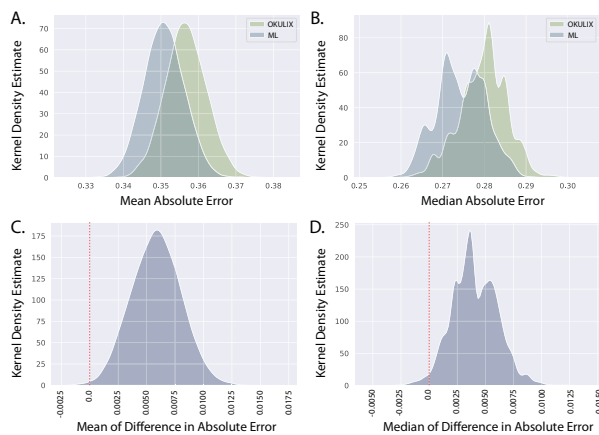
Figure 2 Bootstrap results in the performance comparison dataset. (A) The distribution of the mean absolute error. (B) The distribution of the median absolute error. (C) The distribution of the means of the difference in the absolute errors of OKULIX and the machine learning (ML) method. (D) The distribution of the medians of the difference in the absolute errors of OKULIX and the ML method. The red dashed line marks the location of 0.0.
