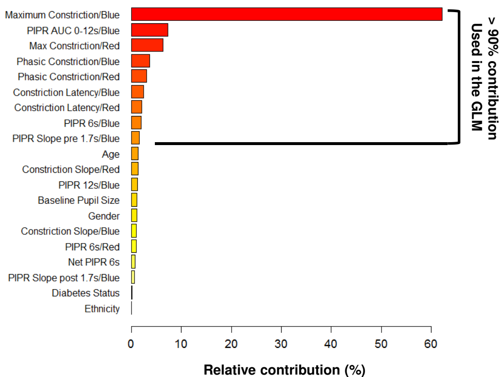
Supplementary Figure 2. Relative contribution of pupillometric, demographic and clinical features for the detection of glaucoma assessed using a gradient boosting machine (GBM) technique. The variables with the highest contribution to the classification model were maximum constriction to blue light (62.2%), PIPR AUC 0-12s (7.3%) and maximum constriction to red light (6.3%). Age and gender contributed 1.4% and 1.1% to the model, respectively, while the relative contributions of diabetes-status and ethnicity were negligible (0 to 0.1%). Top pupillometric contributing features were utilized to develop a generalized linear model for glaucoma classification.
