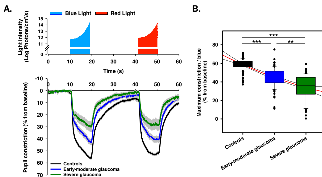
Supplementary Figure 3. Changes in the pupillary light response as a function of the severity of glaucoma. A. Average baseline-adjusted pupillary light responses in patients with early-moderate and severe glaucoma compared to controls. Multiple features of the pupillometric traces were affected by the severity of the disease. B. Gradual decrease in the maximum constriction to blue light as a function of the severity of the disease ( H = 182.4 , P < 0.001 ). The red and black lines represent the linear regression (adjusted R^2 = 0.52 , P < 0.001 ) and 95%CI, respectively. Statistical comparisons between groups were performed using a Kruskal-Wallis One Way ANOVA on Rank. Post-hoc analysis was done pairwise using Dunn's method. **: P < 0.01 ; ***: P < 0.001 .
