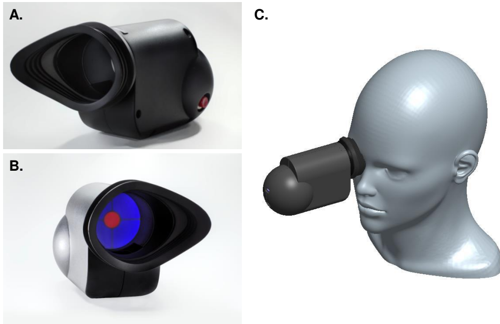
Supplementary Figure 1. Mechanical design of the handheld chromatic pupillometer. A. Photograph showing the overall shape of the device and eye cup. B. Photograph showing one of diverse light stimulation paradigms (central, peripheral, quadrants and full field) allowed by the device. C. Illustration simulating a monocular self-administration of the pupillometric examination procedure by a patient. The fellow eye is typically covered by the patient's hand which is not shown here for illustration clarity purposes. All rights for the photographs and illustration shown in this figure belong to the Singapore Eye Research Institute.
