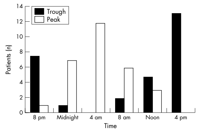
Figure 6 Frequency of CCT peaks and troughs at each time point. Both distribution curves are gaussian, with mean peaks at 4 am and mean troughs at 4 pm.
