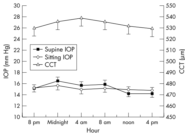
Figure 2 Mean circadian curves of supine IOP (mm Hg), sitting IOP (mm Hg), and CCT (μm). The bars represent standard errors.
