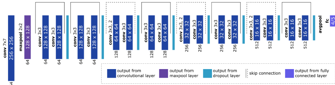
eFigure 3: Architecture of the proposed model. While following a conventional ResNet18 structure, a dropout layer has been added after each ResNet layer. Skip-connections are depicted both as solid and dotted lines, where solid lines represent connections with a constant number of channels and dotted lines implicate a connection where the number of channels increase while the spatial dimensions decrease. The final layer is comprised of four output neurons for FA and five for CF.
